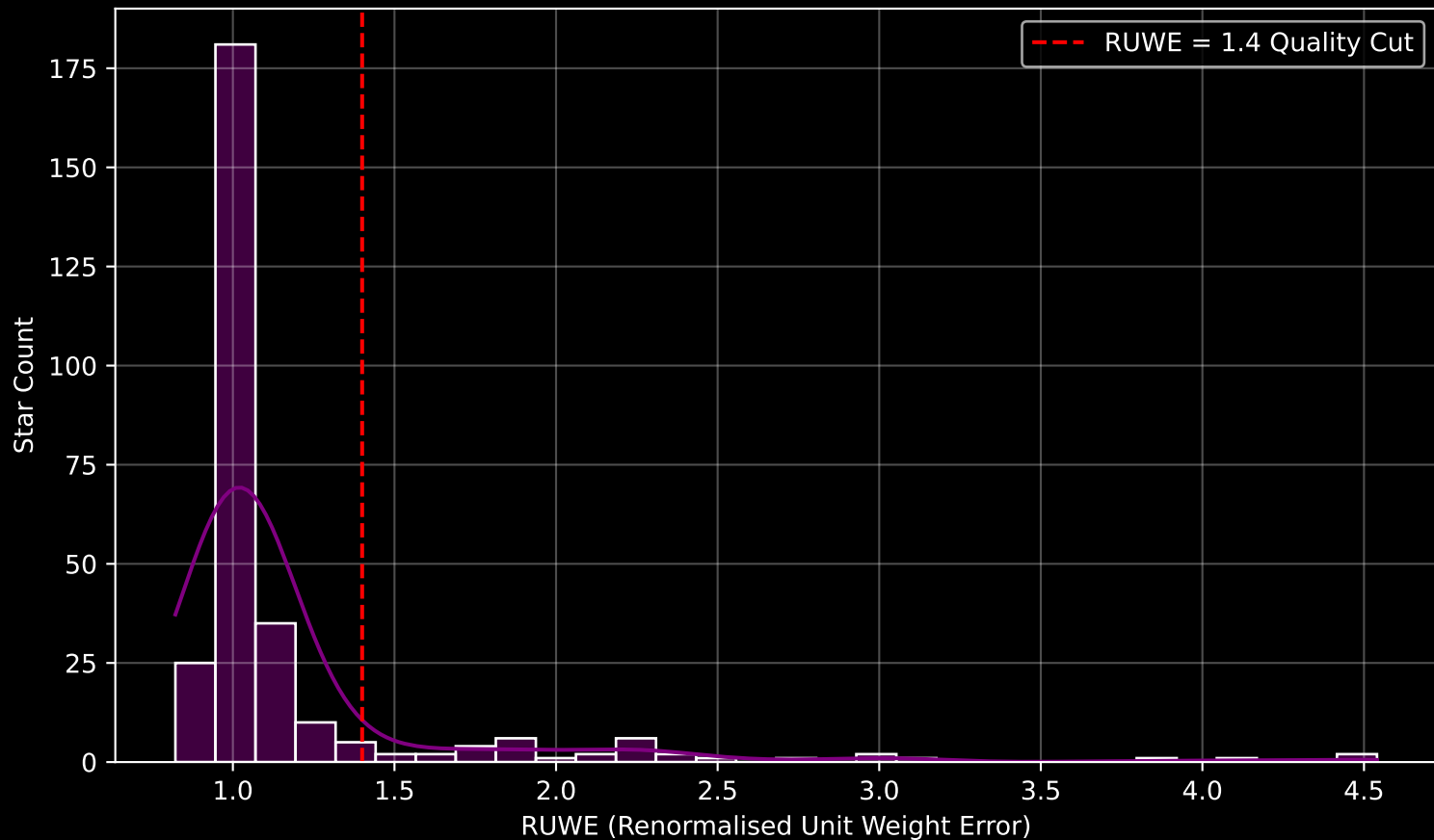
GALAH DR4 Field [586] RUWE Distribution (n= 290)
