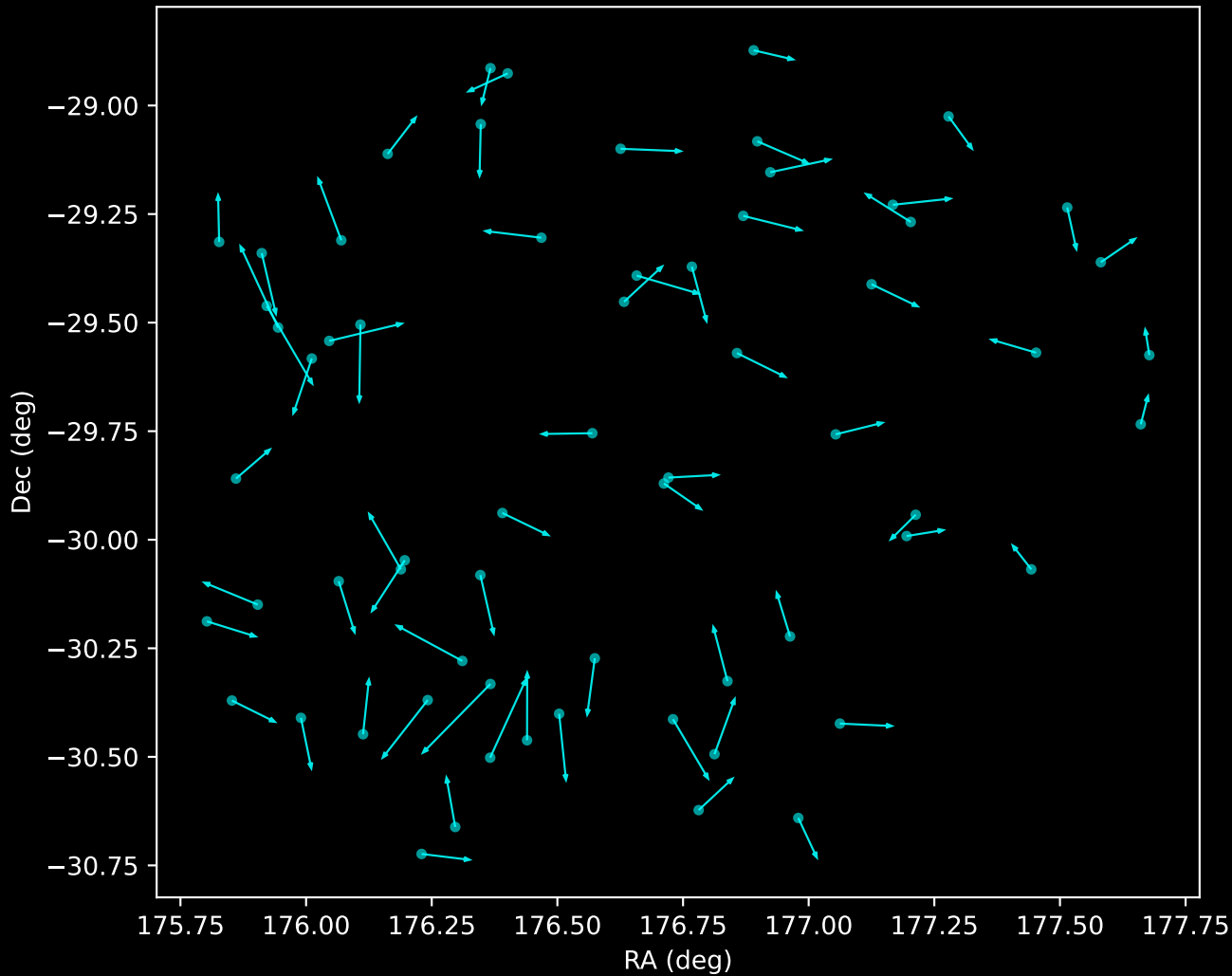
GALAH DR4 Noise Stream Proper Motion Vectors (n=65)
