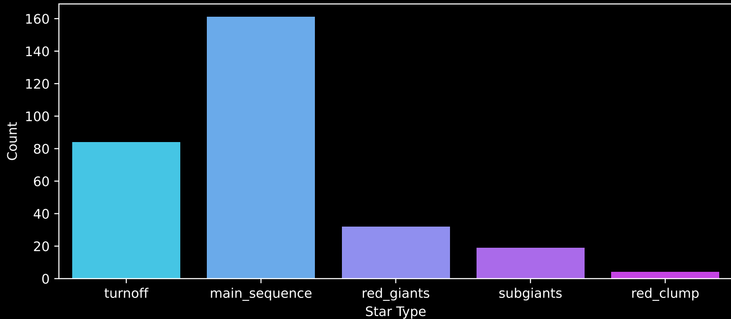
GALAH DR4 Field: [586] Count plot of Star Type
