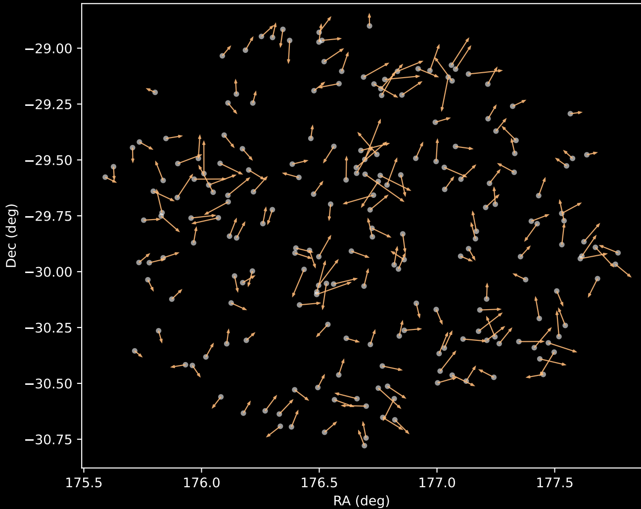
GALAH DR4 Cluster 3 Proper Motion Vectors (n=209)
